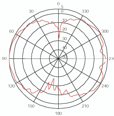
RF Patterns Vertical Cut, typ.
